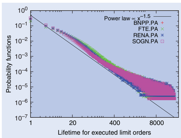
Figure 21. Distribution of the estimated lifetime of executed limit orders.
