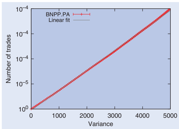
Figure 8. Second moment of the distribution of returns over N trades for the stock BNPP.PA.
