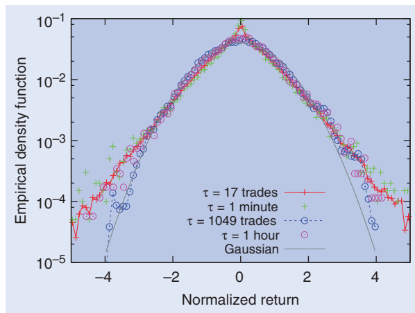
Figure 6. Distribution of log-returns of stock BNP.PA. This empirical distribution is computed using data from 1 April 2007 to 31 May 2008.
