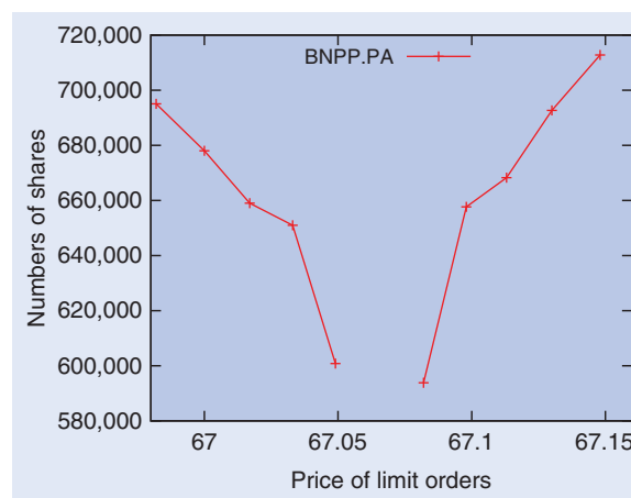
Figure 19. Average limit order book: Price and depth.
