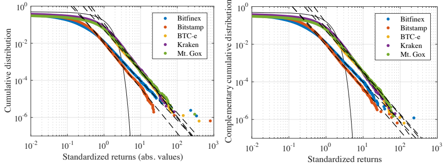
Figure 2: Negative (left) and Positive (right) tails of the cumulative distribution for the Bitcoin returns on the considered exchanges and the time scale of \Delta t = 1 min. The black dashed lines correspond to the fitted power-law distributions for the return tails of the considered exchanges and the black full line is the cumulative distribution function of the standard normal \mathcal{N}(0, 1) .
