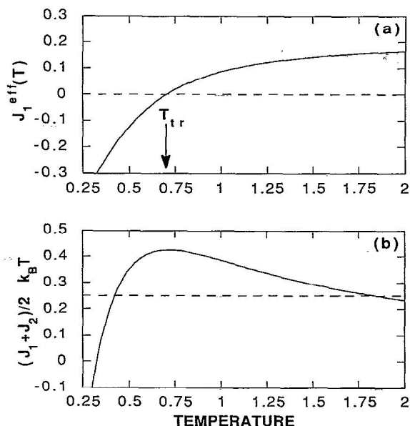
FIG. 3. (a) The effective AB interaction strength J_1^{\text{eff}}(T) as a function of temperature (solid line). The dashed line corresponds to the value zero. The sign of the interaction changes at the temperature where the two lines cross. The temperature and the effective interaction are expressed in units of J . (b) (J_1 + J_2)/2k_B T as a function of temperature (solid line). Also shown is the value of 1/z (dashed line). The two points of intersection correspond to critical points for liquid-gas coexistence.
