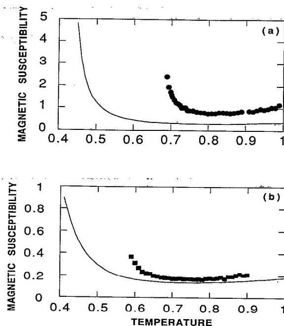
FIG. 7. Magnetic susceptibility from the mean field calculation (continuous lines) and Monte Carlo simulations (data points) for (a) magnetic field h=0 and (b) magnetic field h=0.2 . As in Fig. 8, we see qualitative agreement between mean field and Monte Carlo results. Note that the magnitude of the susceptibility is lower for the higher magnetic field value.
