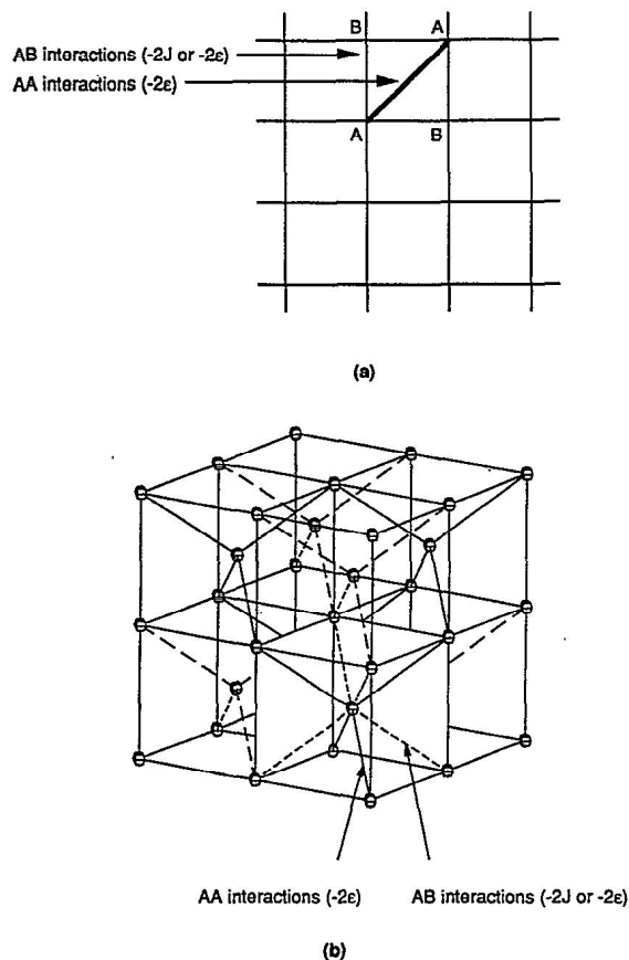
FIG. 1. The division of the lattice into sublattices ( A , B ) and interactions of sites of the same sublattice ( AA interactions) and different sublattices ( AB interactions) are shown (a) for the two-dimensional square lattice, and (b) for the three-dimensional bcc lattice. The A sites are connected by solid diagonal lines to form one of the diamond sublattices. The B sites are connected by long dashed diagonal lines to form the other sublattice. Note that sites at the center of two adjacent cubes belong to different diamond sublattices. The short dashes in the lower right cube indicate AB interactions and should not be confused with the lines representing the division into sublattices. The AA interaction strength is always -2\epsilon while the AB interaction strength is -2\epsilon or -2J depending on the orientational state of the molecule.
