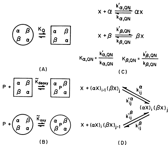
Fig. 1. The special case of the model which we apply here to Hb includes rapid quaternary conformational changes (A, short arrows), rapid phosphate binding (B, short arrows), and slow oxygen binding (C, long arrows). (A) Equilibrium between deoxy and oxy quaternary conformations of unliganded Hb, with equilibrium constant K_Q . (B) Equilibria for phosphate (P) binding to unliganded Hb in the deoxy and oxy quaternary conformation, with equilibrium constants \tilde{K}_{\text{deoxy}} and \tilde{K}_{\text{oxy}} , respectively. (C) Reactions for ligand (X) binding to individual \alpha and \beta subunits in a molecule which is in the Q (deoxy or oxy) quaternary conformation and has N (0 or 1) phosphate molecules bound. For the \alpha subunits, the on and off rate constants are denoted by k'_{\alpha,QN} and k_{\alpha,QN} , respectively, and the equilibrium constant by K_{\alpha,QN} . Similar notation is used for the \beta subunit. For a fixed phosphate concentration this model is equivalent to the extended Adair model (2) shown in (D). The overall rates k_{ij}^{\alpha} , k'_{ij}^{\alpha} , k_{ij}^{\beta} , and k'_{ij}^{\beta} are functions of the rate constants and equilibrium constants defined above.
