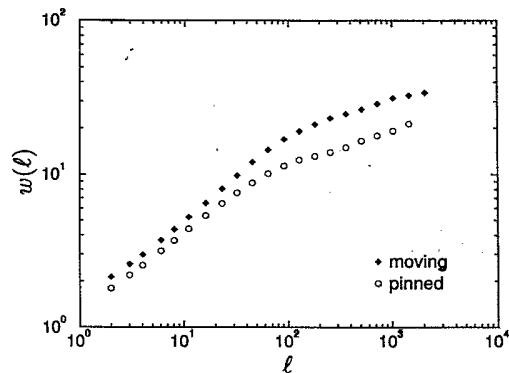
FIG. 3. Experimental local width w for the pinned and the moving interfaces in 1 + 1 dimensions. It is visually apparent that the moving interface has a larger width and a different roughness exponent than the pinned interface.
