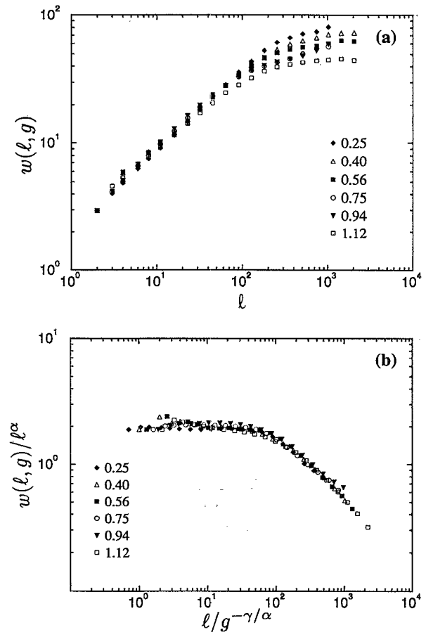
FIG. 19. Experimental results for the width w(\ell, g) of the pinned interface. (a) The widths for several values of the gradient g (in units of g_0 ). The values of g were calculated as described in the text; the error in these values is smaller than 10%. The widths were corrected by a multiplicative factor to make them coincide for the smallest \ell . (b) The same experimental results, plotted in the scaling form of Eq. (5.4), using the values of the exponents from (5.13).
