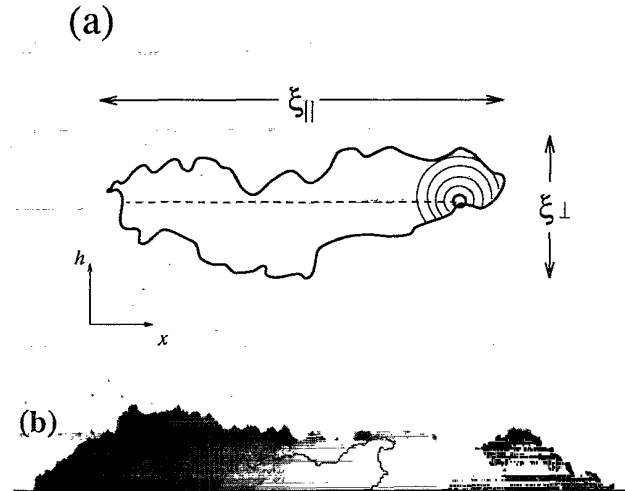
FIG. 10. Illustration of the dynamics of the DPD model for 1+1 dimensions. (a) Schematic representation of a region defined by two pinning paths. The heavy circle indicates the origin for the invasion, the thin arcs represent the positions of the invading front at successive times, and the dashed line represents schematically the path for the invasion. (b) Simulation results for invasion after 2^{10} time steps starting from a single cell near the center. We show the invaded region at a sequence of times that are multiples of 128. Regions invaded at later times are displayed in darker shades of gray. The path from the origin to the latest invaded point is shown in black. Although this path displays some fluctuations in the vertical direction, they can be disregarded since \nu_{\parallel} > \nu_{\perp} , so as p \rightarrow p_c , \xi_{\perp}/\xi_{\parallel} \rightarrow 0 . Thus the distance propagated by the invading front is proportional to time. Since t_x \sim \ell , we can conclude that z = d_{\min} = 1 .
