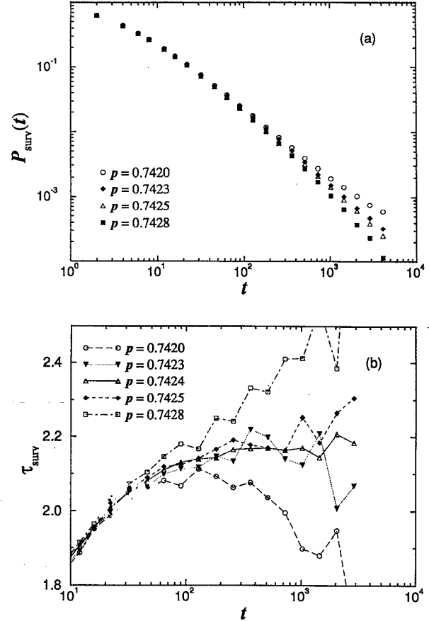
FIG. 14. Distribution of survival times for avalanches P_{\text{surv}}(t) for 2+1 dimensions. The system size is 2048 and 10^6 avalanches were produced for each probability. In (a) we show data for several probabilities close to the critical value. The straight part of the distribution can be well fitted to a power law with exponent 2.18. In (b) we show the consecutive slopes of the data in (a). The figure makes clear that we can predict with great precision the value of p_c and the error of the estimate.
