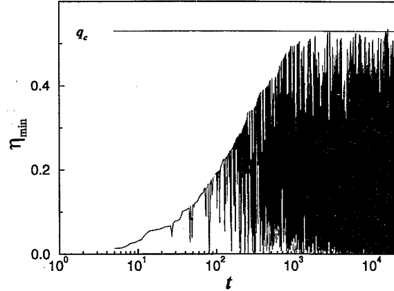
FIG. 17. Evolution with time of \eta_{\text{min}} . Every local maximum defines the end of an avalanche and the beginning of another. Regions with monotonic growth indicate that the avalanches have size 1. After the transient period, the critical state is reached and the maxima become equal to q_c = 1 - p_c .
