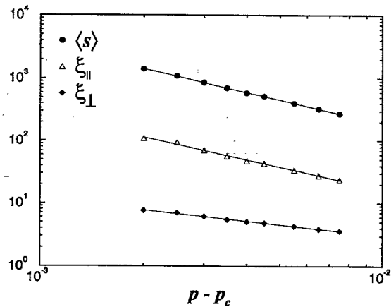
FIG. 16. Scaling of the average size s and parallel and perpendicular correlation lengths of the avalanches for 2 + 1 dimensions. These quantities were calculated according to the method described in Appendix A. Good power-law fitting was found with the exponents given in (4.16).
