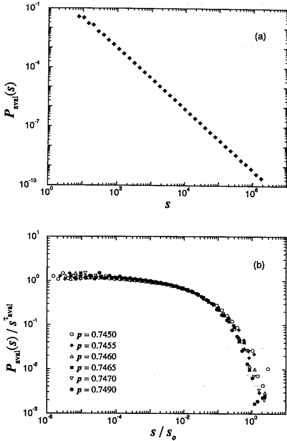
FIG. 15. Distribution of avalanches size P_{\text{aval}} for 2 + 1 dimensions. The system size is 2048 and 10^6 avalanches were produced for each probability. In (a) we show the data for the critical probability; a good power-law fit can be done with an exponent 1.51. (b) shows a data collapse, according to (4.2), for several distinct probabilities close to p_c .
