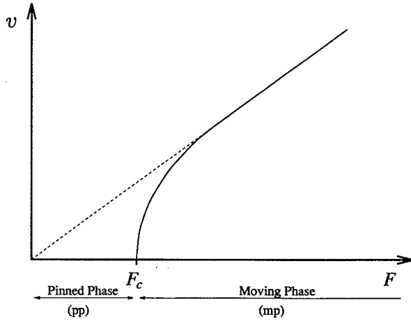
FIG. 1. Depinning transition. In the “pinned phase” (PP) F < F_c , the velocity of the interface is zero. In the “moving phase” (MP) F > F_c , the interface moves with a constant average velocity v . The velocity plays the role of the order parameter of the transition.
