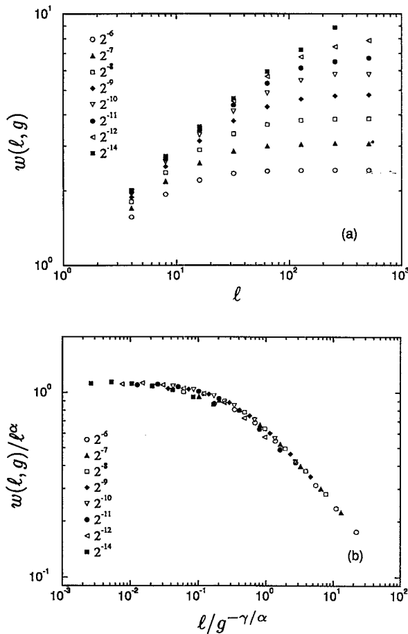
FIG. 18. Simulation results for the width w(\ell, g) of the pinned interface in 2 + 1 dimensions, where g is the gradient in the density of blocked cells. (a) The widths for several values of the gradient (averaged over 128 runs for each value of the gradient). (b) The same simulation results, plotted in the scaling form of Eq. (5.4), using the values of the exponents from (5.10).
