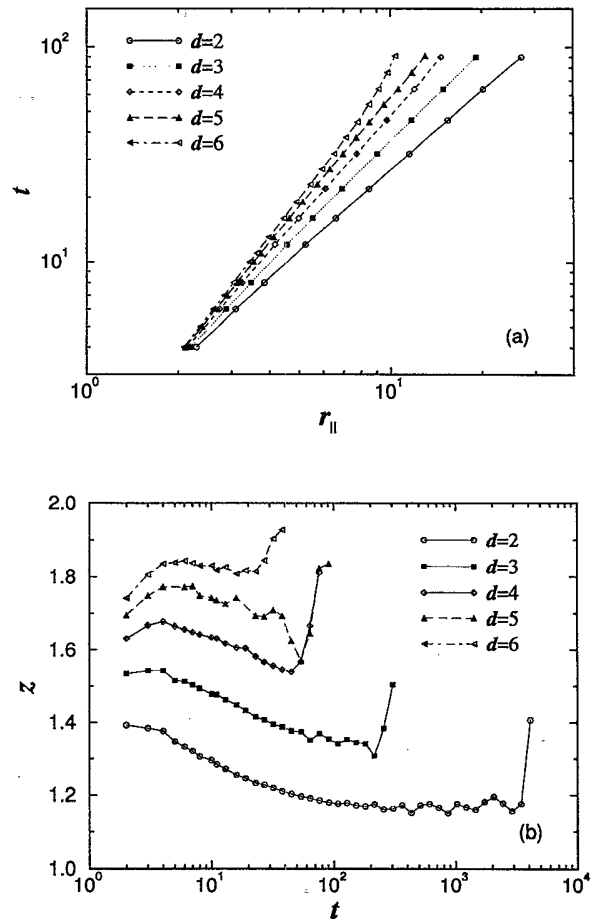
FIG. 12. (a) Scaling with time of the horizontal length of a DPD cluster in d + 1 dimensions grown from a single cell. Shown is a plot of time t as a function of r_{\parallel} , which is the average of the parallel components of the radius of gyration of the shell. The asymptotic slope is z . (b) Consecutive slopes analysis of the data displayed in (a). Note that, after some transient behavior, a transition to a power-law scaling occurs. For higher dimensions, the power-law scaling is affected by finite-size effects for larger times.
