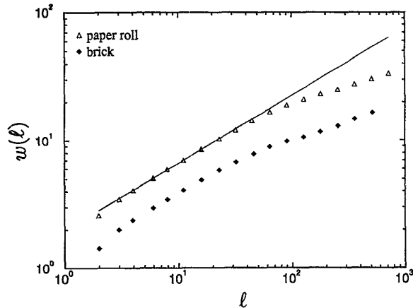
FIG. 5. Scaling of the local width w with \ell for the experiments in 2 + 1 dimensions. The curve for the paper roll results from averaging over 13 different paper sheets and the one for the Oasis brick results from averaging over 9 different sections.
