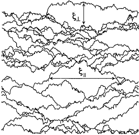
FIG. 13. Successive series of pinned interfaces for the DP model with L = 400 and p = 0.5 > p_c . We show the boundaries of avalanches, produced by removing a randomly chosen blocked cell from the previously pinned interface. The correlation lengths \xi_{\parallel} and \xi_{\perp} displayed describe the typical size of the avalanches.
